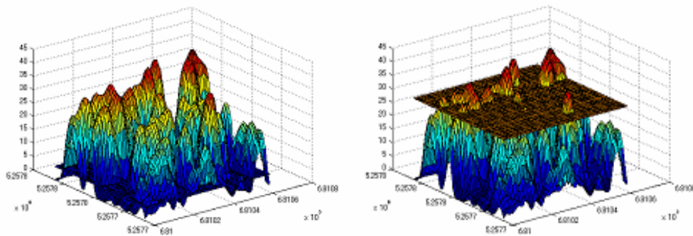
Figure 1. The marching sliced plane used to identify the local peaks of the surface. The smooth surface was created by the local maxima of LIDAR points. The starting plane is shown in the left and the plane at the intermediate step is shown in the right.
